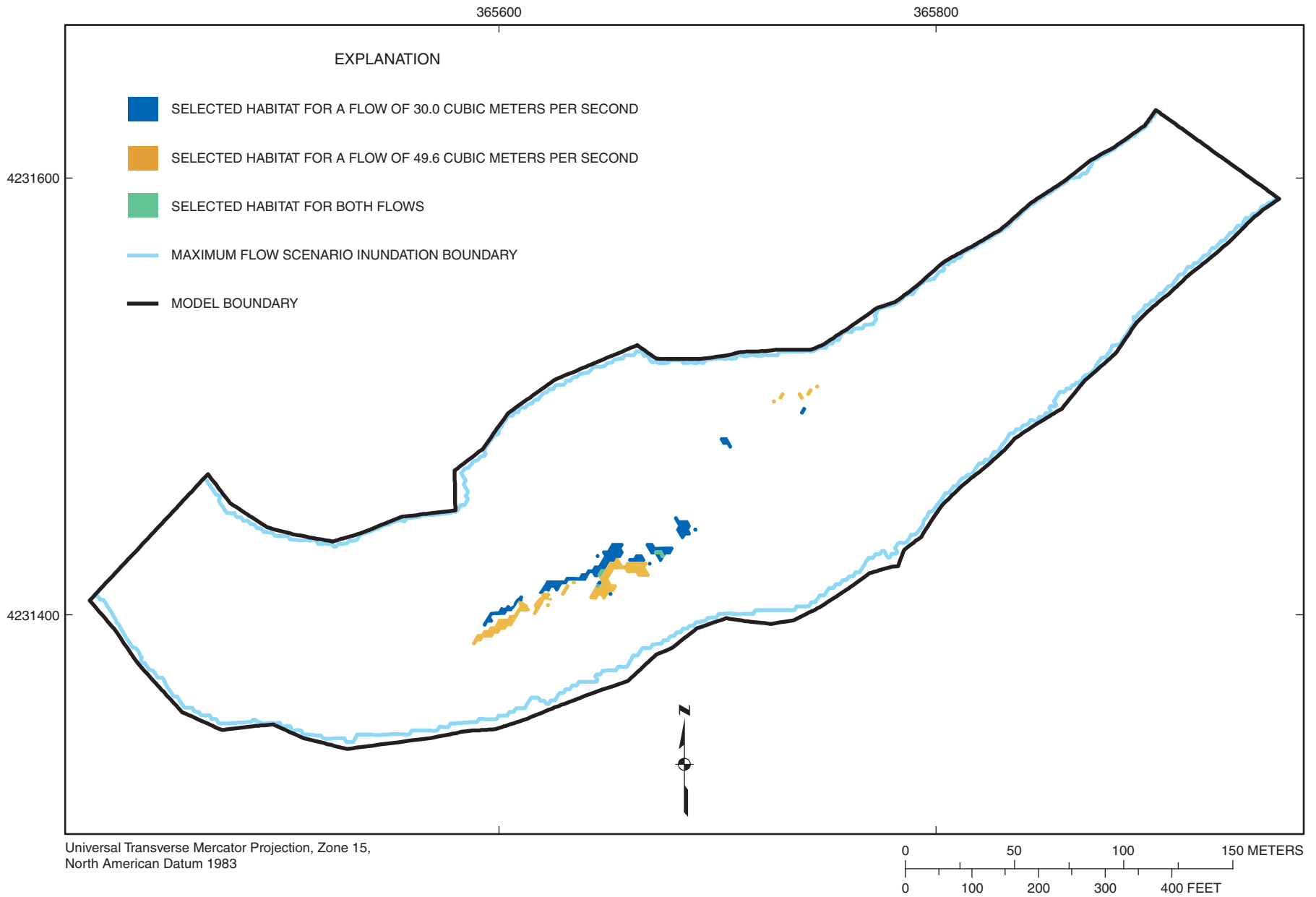
Figure 4-75. Selected habitat area distribution for habitat category 19 (stonecat) at flows of 30.0 and 49.6 cubic meters per second at Marais des Cygnes River site MDC2.
